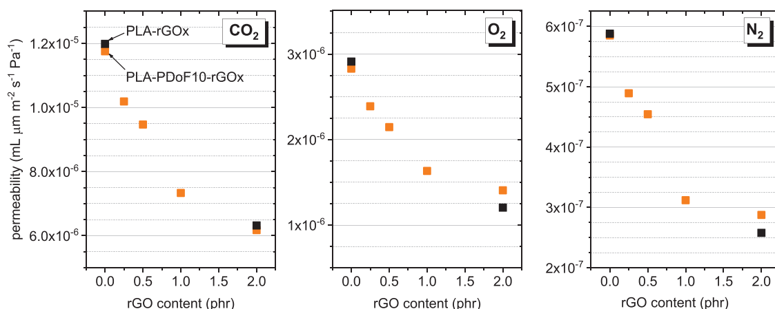
Figure 4. Permeability to CO 2 , O 2 , and N 2 as a function of the rGO content for the samples PLA-rGOx and PLA-PDof-rGOx. Experimental indeterminations are inside the size of the symbols. Data from ref.[15] PDof, poly(dodecylene 2,5-furandicarboxylate); PLA, poly(lactic acid); rGO, reduced graphene oxide.
