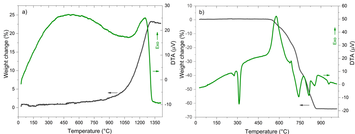
Fig. 8. TG/DTA under air flux: a) pure ceramic aerogel; b) AS composite.
